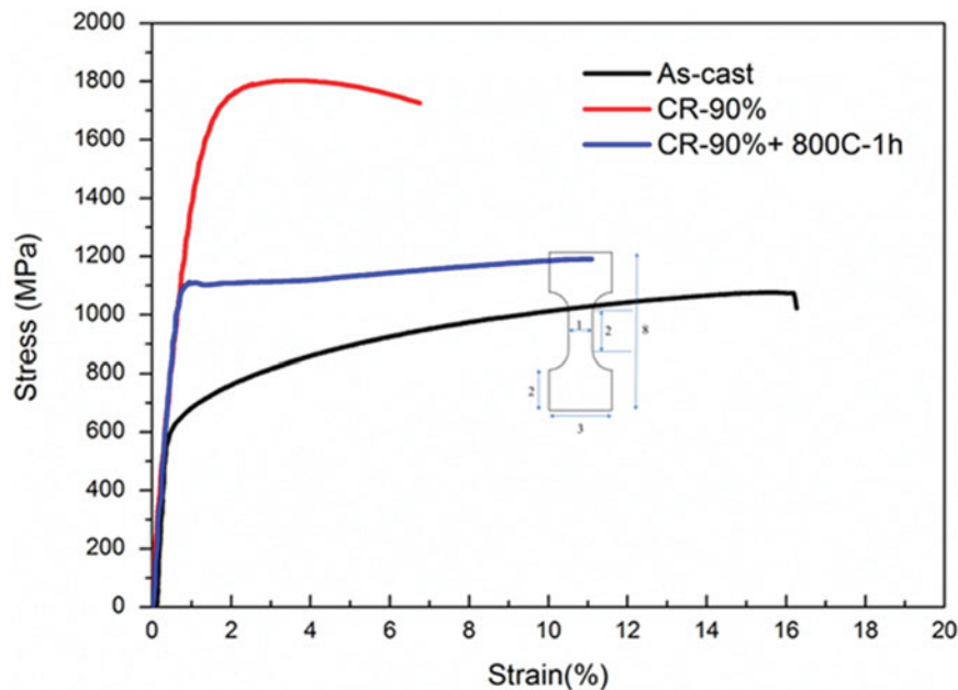
Figure 4. (Colour online) Engineering stress–strain curves of the AlCoCrFeNi 2.1 EHEA in the as-cast, cold-rolled and annealed conditions. The dimensions of the tensile specimen is shown inset (all dimensions in mm).
