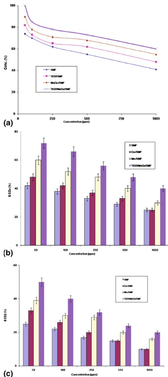
Figure 1. Influence of SMF modification and benzene concentration on (a) conversion, (b) selectivity to CO x and (c) selectivity to CO 2 at 230 J/l.
